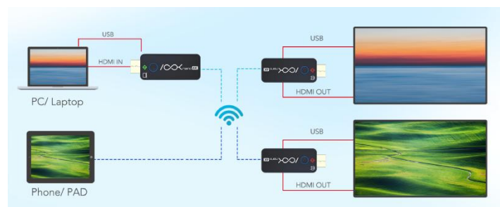
ASK nano 4K System Connection Diagram 2
