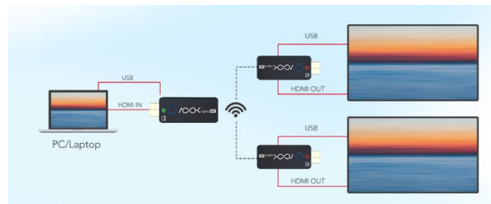
ASK nano 4K System Connection Diagram 1
